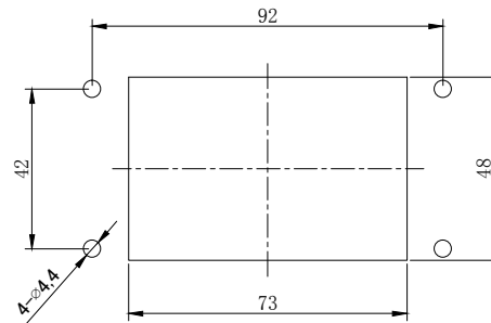
面板开孔图 Panel cut out
